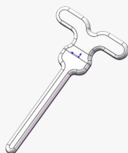
T Type Pin A10-51
